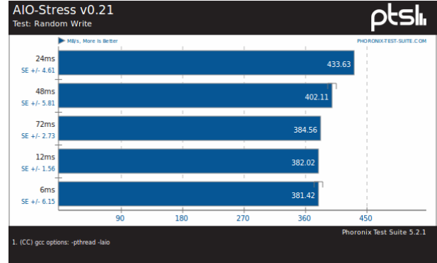
Figure 4: Bar chart of performance for latency variable.
